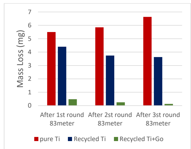
Figure 4. Comparison of wear Values of Samples
